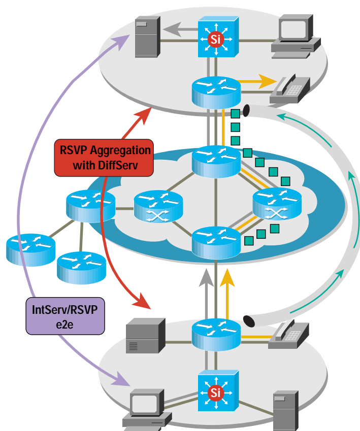
Figure 7 IntServ Over DiffServ Tomorrow
