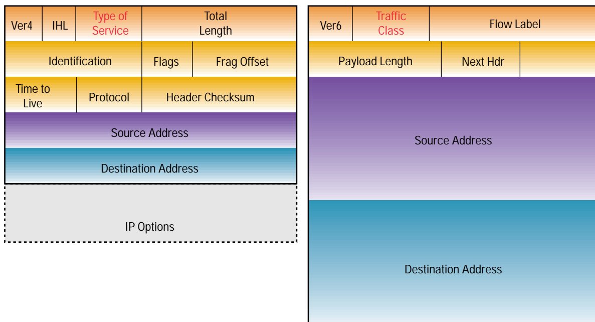
Figure 1 IPv4 and IPv6 Headers
